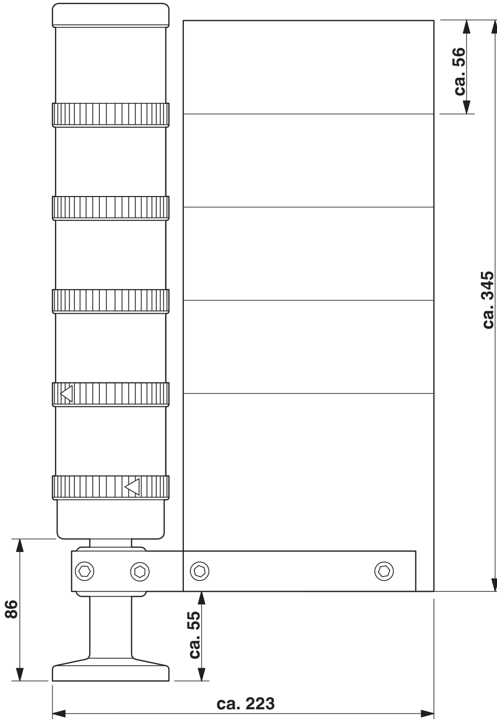
Dimensional drawing
